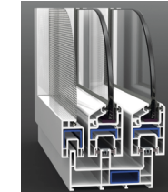
Double Rail with Screen Sash
